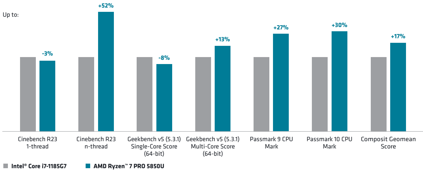
CPU Performance
